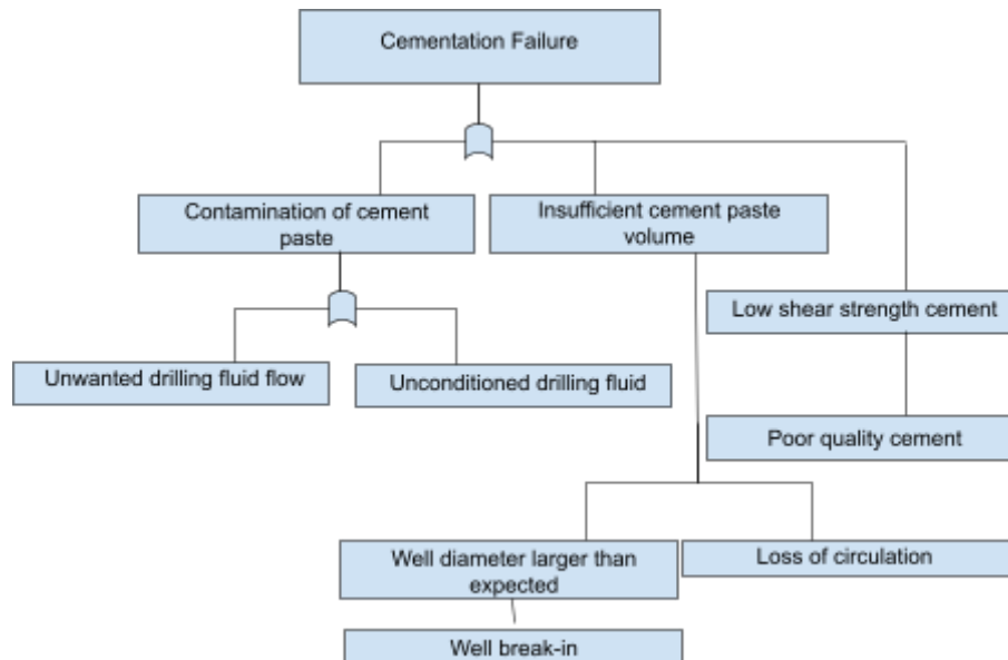
Figure 2. FTA of Failure to cement.
